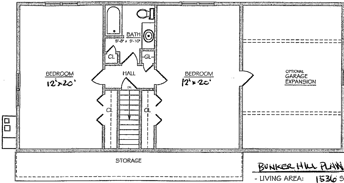
SECOND FLOOR PLAN SQ. FT. LIVING AREA
