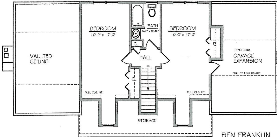
SECOND FLOOR PLAN 654.5 SQ. FT. LIVING AREA
